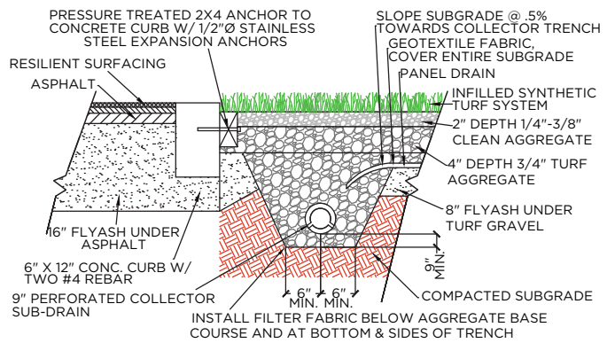
CURB
