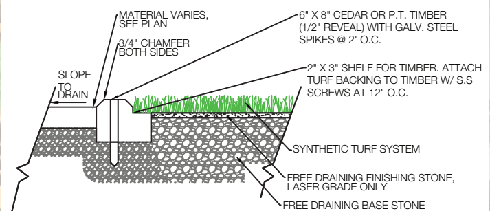
NAILER BOARD
