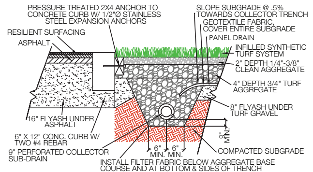
CURB
